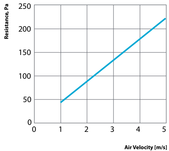
Airflow Resistance
